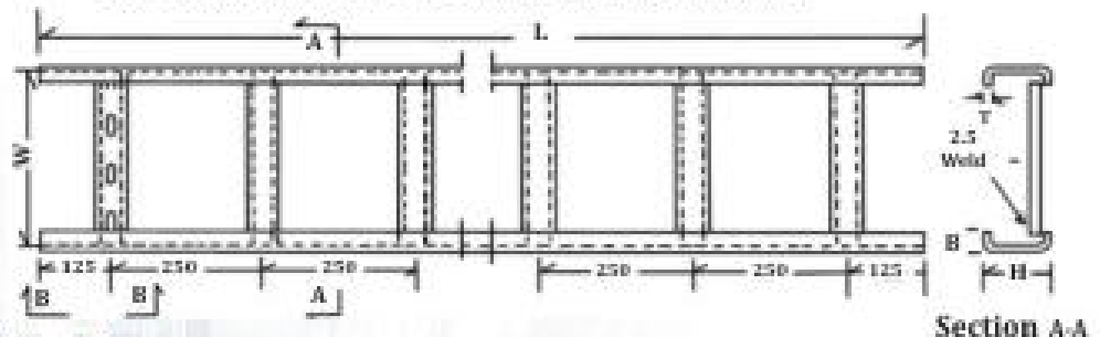
Typical Lay Out for Ladder Type Cable tray for length 2500mm
